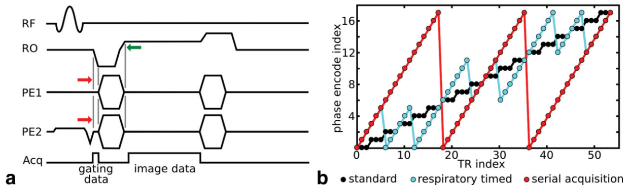
FIG. 1. 3D image acquisition sequence. a : All images were acquired using a modified 3D gradient echo sequence. The phase encoding gradients on both axes (PE1 and PE2) were shifted to a slightly later time (red arrows) to permit acquisition of gating data during the initial portion of the readout (RO) dephasing gradient. A shift equal to the gradient rise time (200 \mu s on our system) avoids time cost by overlapping the falling edge of the phase encode gradient with the rising edge of the readout gradient (green arrow). b : The phase encode acquisition order during the scan was prescribed in one of three ways according to the application. The standard ordering (black) used repeated acquisition of each phase encode until all averages/repeats were collected and then proceeded to the next phase encode. Respiratory-timed encoding (cyan) was designed for retrospective respiratory gating and acquired phase encode averages/repeats every \sim 400–600 ms (about one-half a respiratory period) to ensure at least one acquisition for each phase encode with minimal respiratory effects. This was achieved by acquiring N consecutive phase encodes together and then repeating the set for averages/repeats (b: shows N = 6 with three repeats, typical imaging scans in this work used N \approx 8 with three repeats). For in utero imaging, phase encodes were incremented linearly (red) until a full image was acquired, and then the entire image was repeated (serial acquisition). In (a), RF = radiofrequency, Acq = acquisition, RO = readout gradient, PE1 = first phase-encode gradient, PE2 = second phase-encode gradient.
